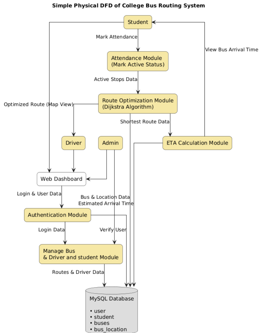
Figure 3.10: Physical DFD
